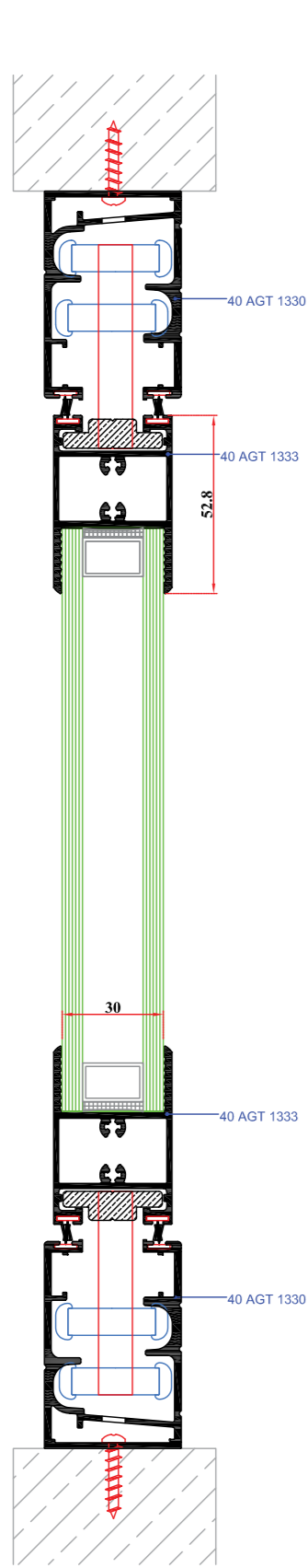
1 NOLU DETAY
