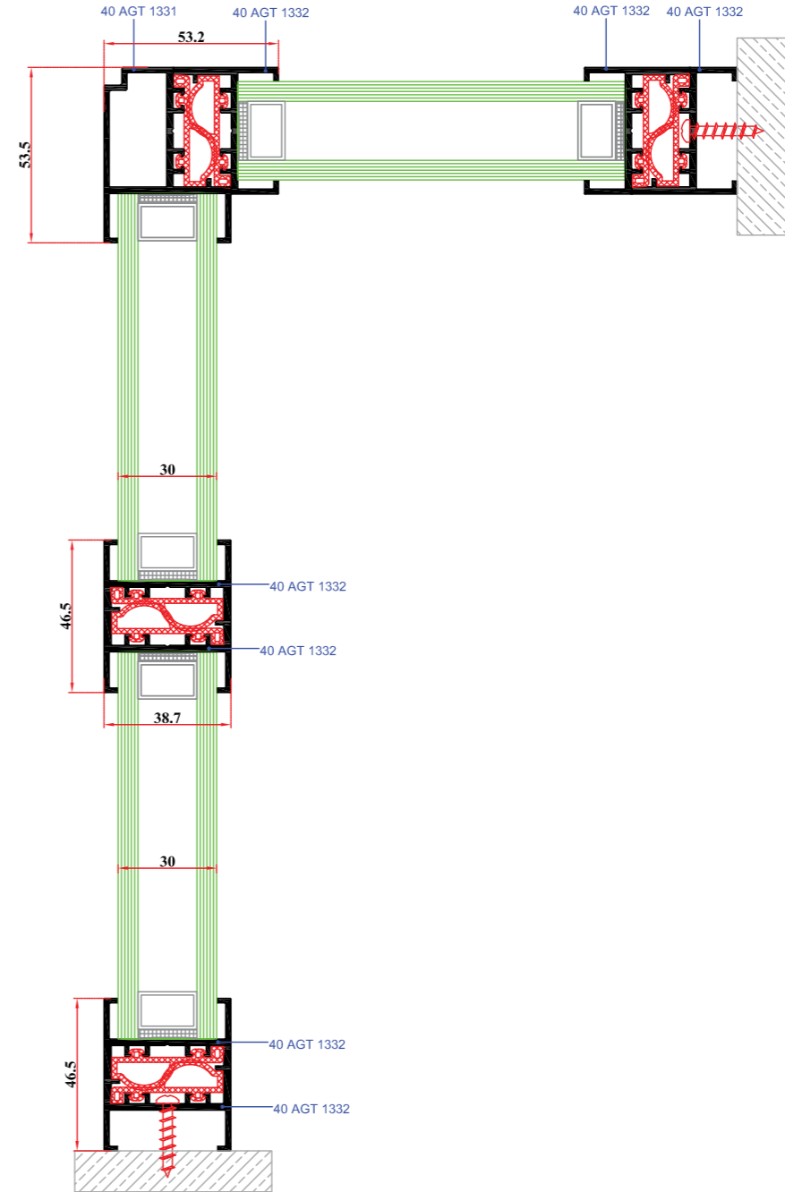
1 NOLU DETAY
