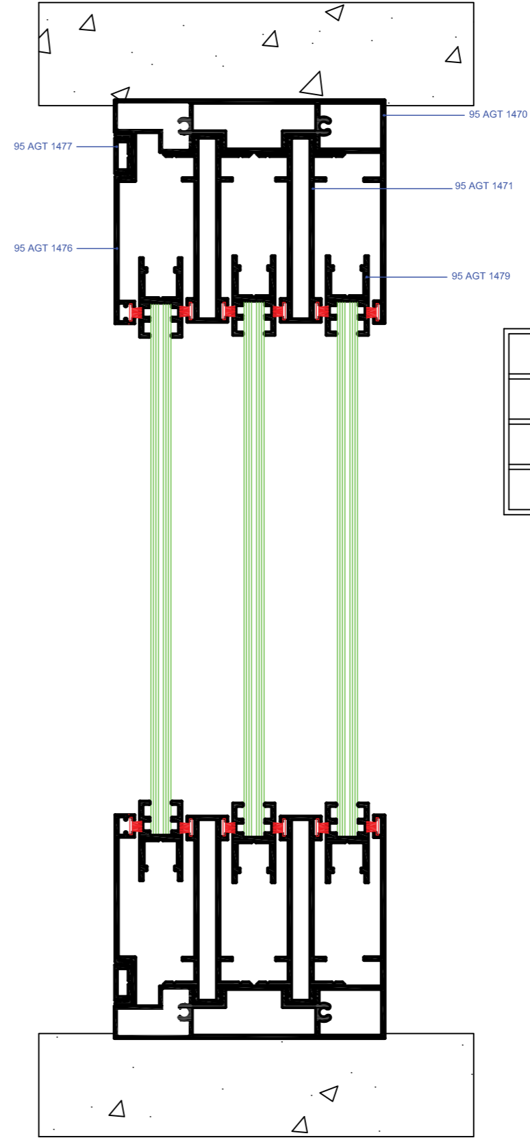
1 NOLU DETAY
